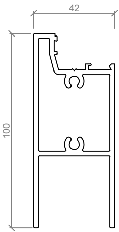
ASL 645 100mm TOP & BOTTOM RAIL
