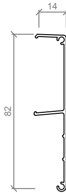
ASL 180 KG TOP TRACK PELMET
