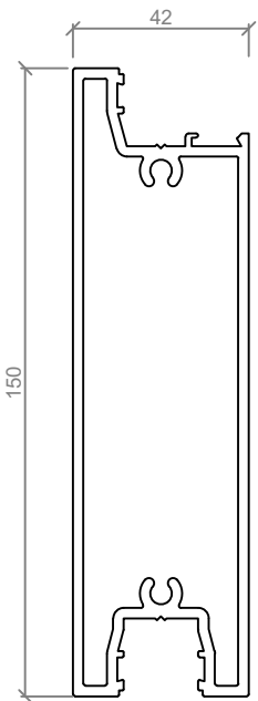
ASL 776 150mm TRANSOM & BOTTOM RAIL
