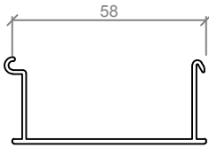
ASL 352 PELMET CLOSER
