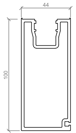
ASL 665 100mm CLOSING STILE
