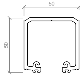
ASL 250KG TOP TRACK
