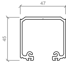
ASL 180 KG TOP TRACK
