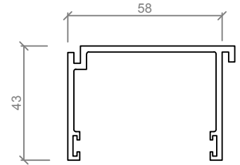
ASL 100 HEAD GUIDE (MATING)
