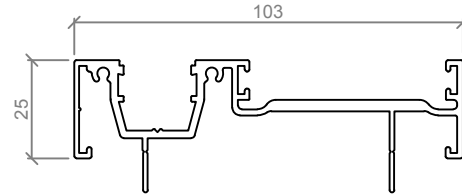
ASL 353 VERTICAL STARTER
