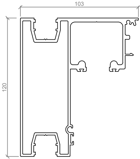
ASL 350 TOP ROLLER TRACK WITH FIXED GLAZING
