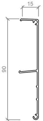
ASL 250KG TOP TRACK PELMET
