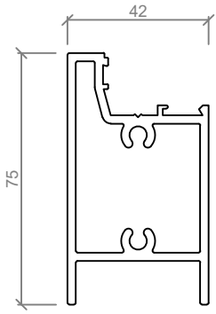
ASL 605 75mm TOP & BOTTOM RAIL
