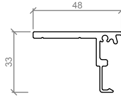
ASL 357 PELMET ADAPTER
