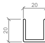
GUIDE CHANNEL
