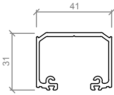
ASL 120 KG TOP TRACK
