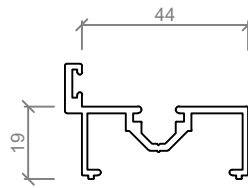
ASL 225 GLAZING MULLION
