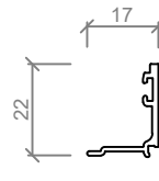
ASL 541 GLAZING BEAD
