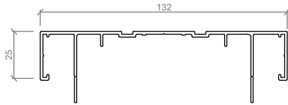
ASL 420 132mm REBATED HEADSECTION
