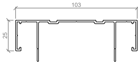
ASL 400 103mm REBATED HEADSECTION
