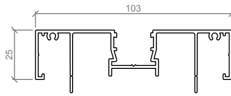
ASL 546 103mm POCKET HEADSECTION
