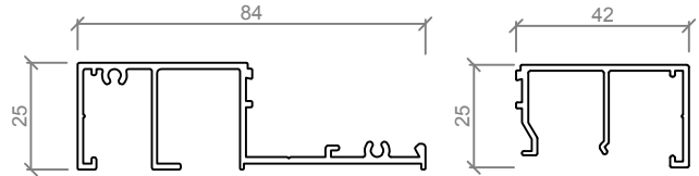
ASL 588 GLAZING BAR
