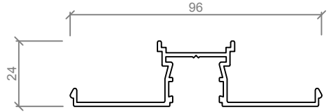
ASL 543 POCKET STARTER CAP
